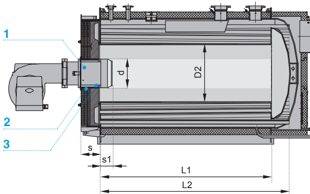
Burner installation
