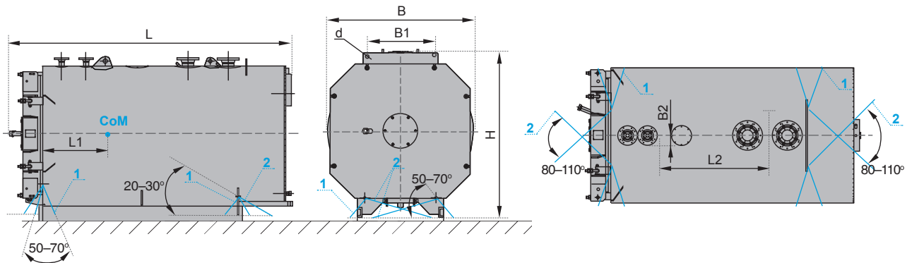
Diagram of transportation of boilers with a heat output of 5400–16500 kW
