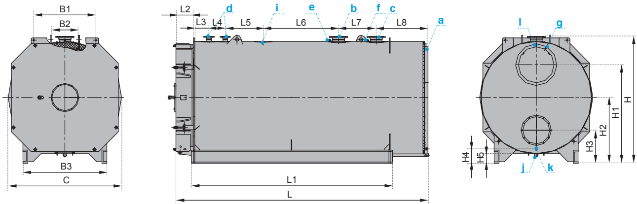
Overall and connecting dimensions of boilers with a heat output of 5400–16500 kW
