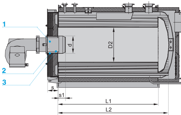
Burner installation
